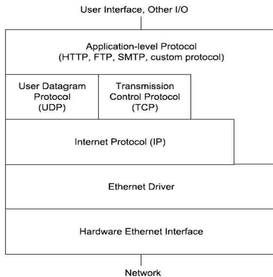
Fig-1: Network Protocol Stack
