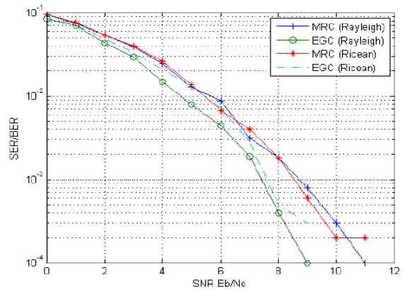
Fig. 8. Error plots for MISO (4 × 1) configuration
