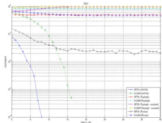
Fig. 5. Error Plots for SISO configuration
