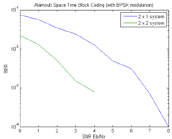
Fig. 9. Error plot for a 2 × 1 and 2 × 2 system
