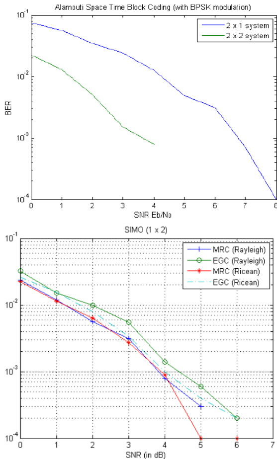
Fig. 7. Error Plots for SIMO (1 × 2) configuration
