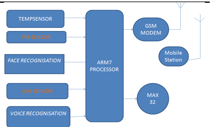
Fig.6. System block Diagram
