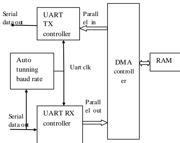
Fig.1. block diagram of UART IP soft core based DMA
