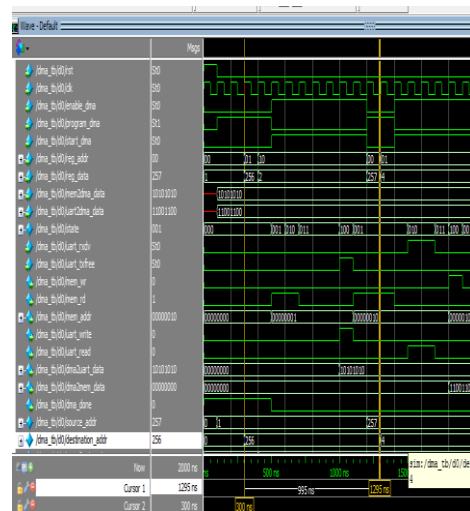
Figure 7: DMA waveforms
