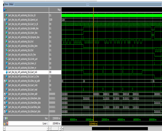
Figure 2: UART IP Soft core top level waveforms.
