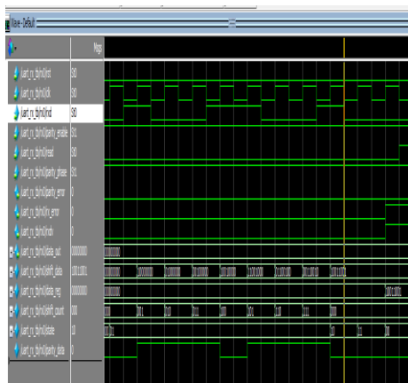
Figure 5: UART Receiver waveforms
