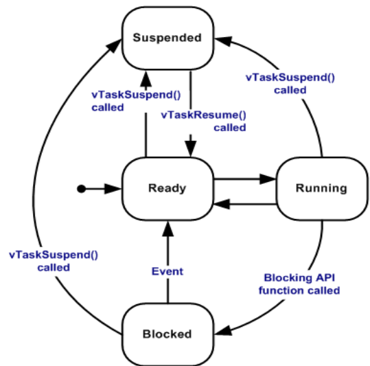
Figure4. Life cycle of a task
