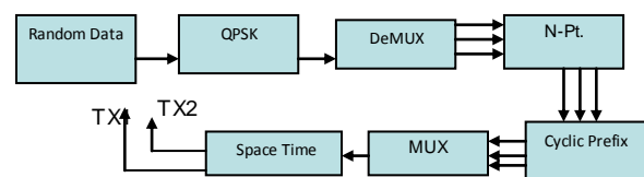
Fig. 4 MIMO-OFDM Transmitter
