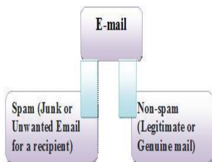
Fig. 1 Email Types
