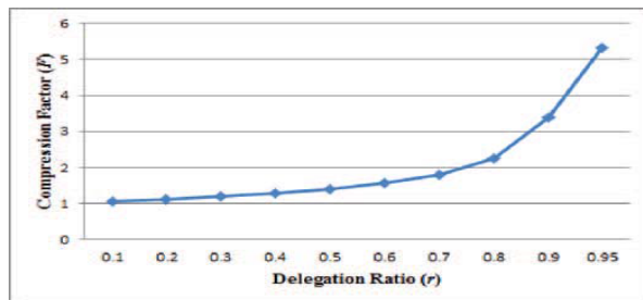
(A) Compression achieved by the tree-based approach for delegating different ratio of the classes
