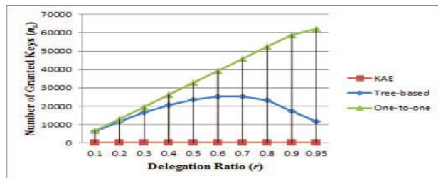
(B) Number of granted keys ( n_a ) required for different approaches in the case of 65536 classes of data
