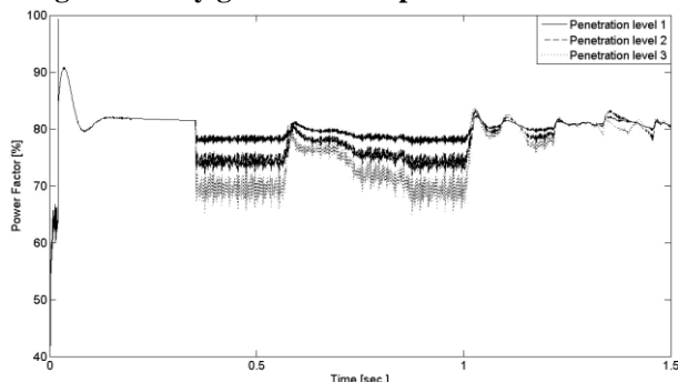
Fig. 11. Utility grid2 power factor at bus 2.
