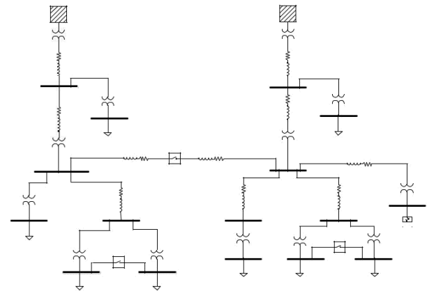
Fig. 3. Single-line diagram of the 16-bus test system.
