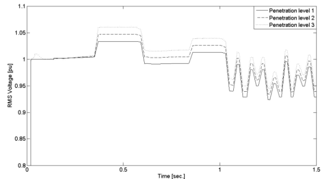
Fig. 12. System voltage magnitude at bus 6.
