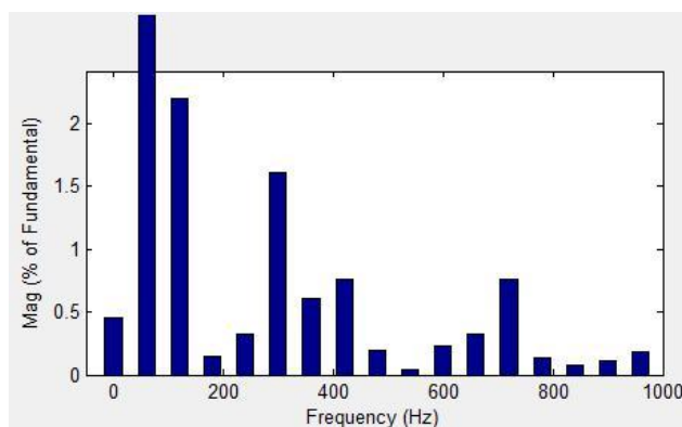
Fig. 16. Current harmonic spectrum at bus 11.
