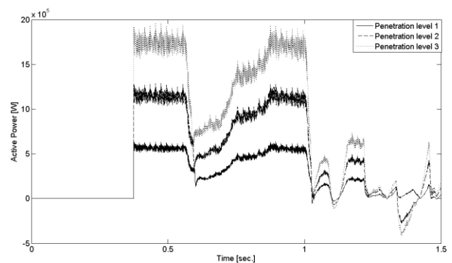
Fig. 5. Injected power by PV system at bus 11.
