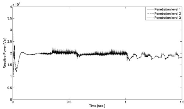
Fig. 7. Utility grid1 reactive power at bus 1.
