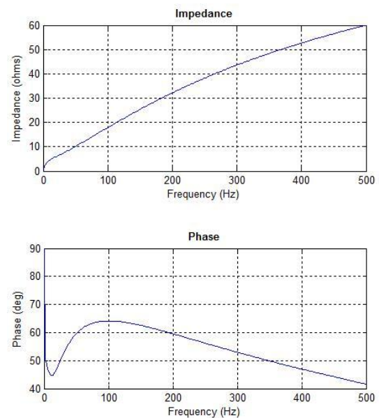
Fig. 17. System impedance vs. frequency curve.
