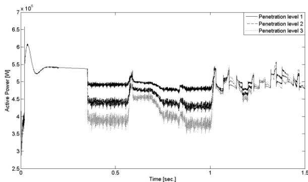
Fig. 9. Utility grid2 active power at bus 2.
