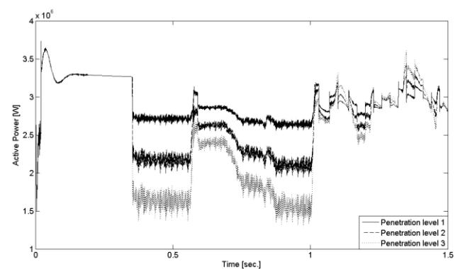
Fig. 6. Utility grid1 active power at bus 1.
