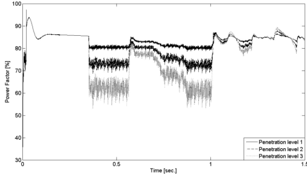
Fig. 8. Utility grid1 power factor at bus 1.
