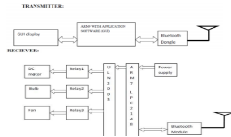
Fig -1: Block diagram of Bluetooth Based Home Automation and Security System Using ARM9
